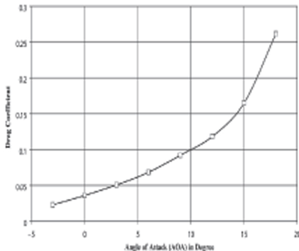
Figure 10: Variation of Drag Coefficient with Angle of Attack for Aerofoil Shaped Fuselage Model at 40 m/s [6].
