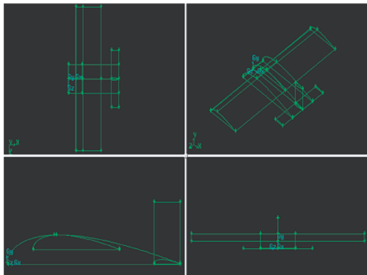
Figure 4: Wire-frame Views of Aerofoil Shaped Fuselage Model [6].
