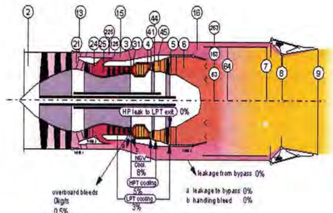
Figure 7 : Variable Cycle Engine
