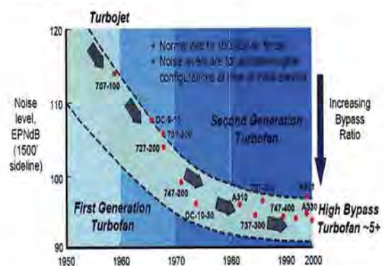
Figure 3: Progress in jet engine noise reduction [4]
