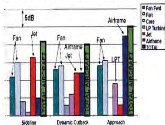
Figure2: Example for noise source breakdown for high by pass ratio/low fan pressure ratio
