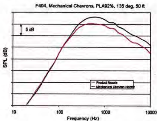
Figure 6: SPL (Sound Pressure Level) vs. Frequency
