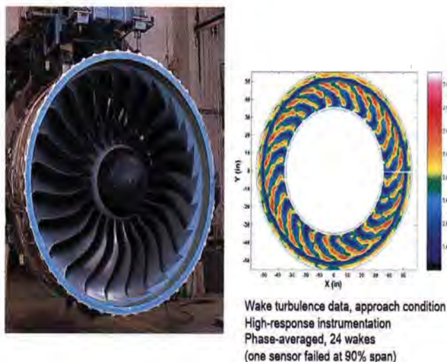
Figure 8: GP7000 Swept Fan
