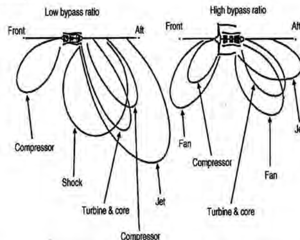
Figure 1: Noise sources for engines. Engine bypass ratio has a large effect on noise characteristics (Pinker, 1991)[2]
