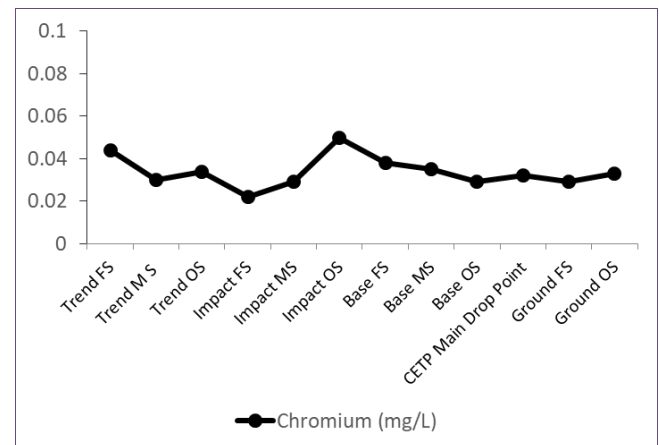
Figure 6: Concentration of Cr^{6+} in water bodies at different sampling locations in Savar area
